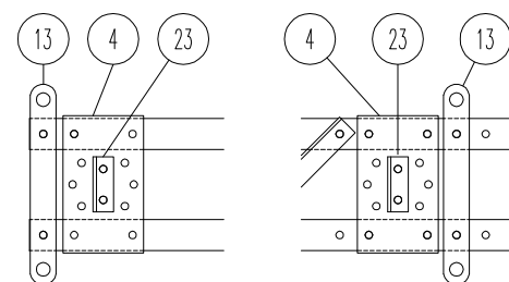
DOWNLEAD ATTACHMENT PLATE CROSSARM POSITION
